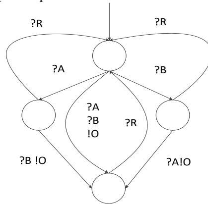
Fig. 6 State machine of ABRO
