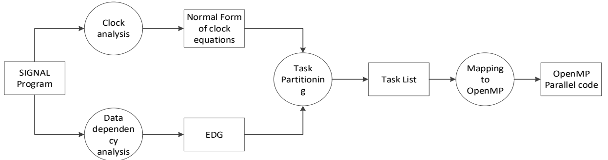
Fig. 5 Process of Parallel-Code Generation from SIGNAL Specification to OpenMP
