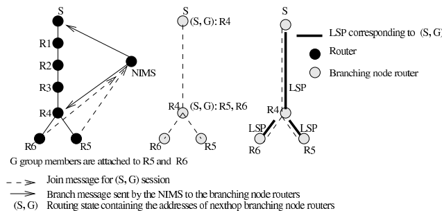
Figure 1: The MPLS multicast tree construction
