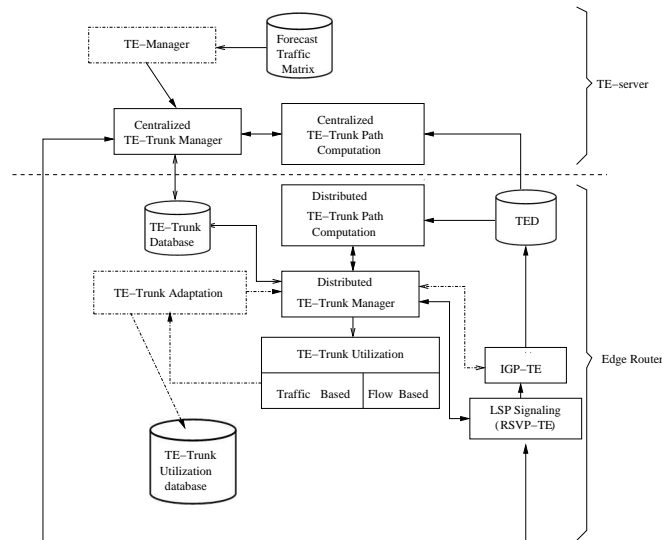
Fig. 3. Hybrid MPLS-TE Approach
