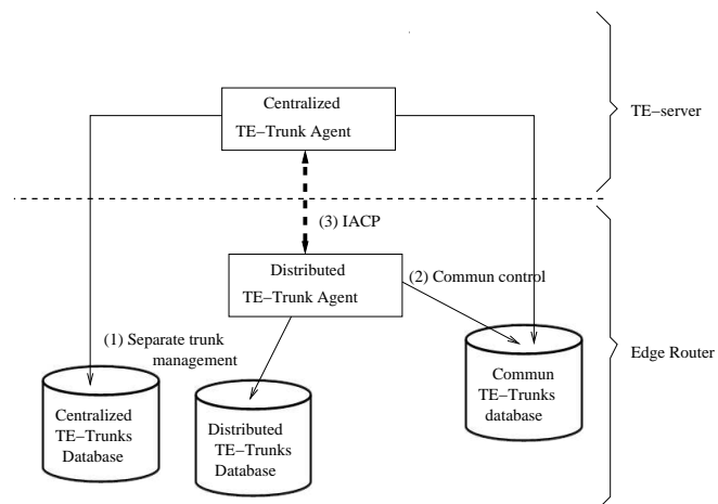
Fig. 4. TE-Trunks management
