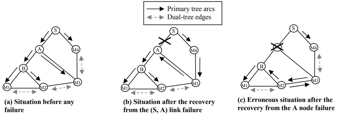
Fig. 2. Dual-tree protection
