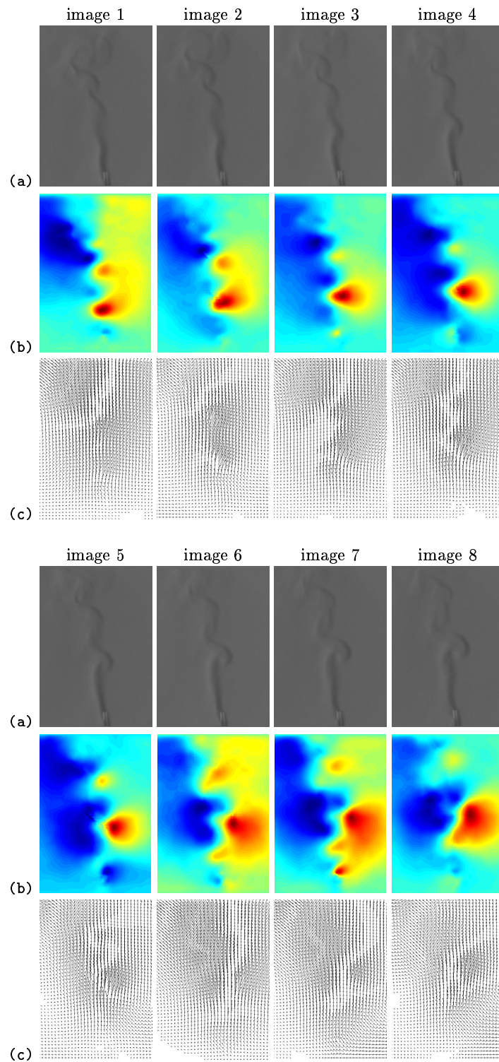
Fig. 4. natural convection. sequence of (a) images, (b) estimated vorticity maps and (c) estimated displacement fields
