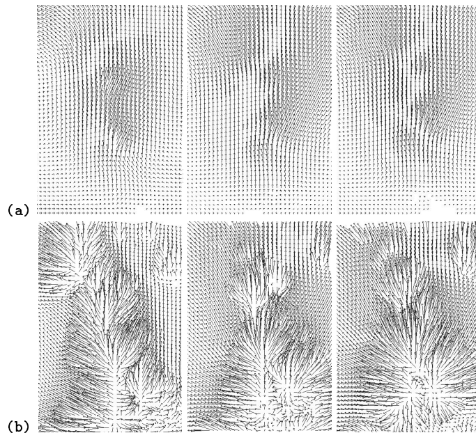
Fig. 3. natural convection. comparison between the estimated displacement fields obtained on images 2,3,4 with (a) our estimator and (b) the fluid dedicated estimator of Corpetti et al. [14].
