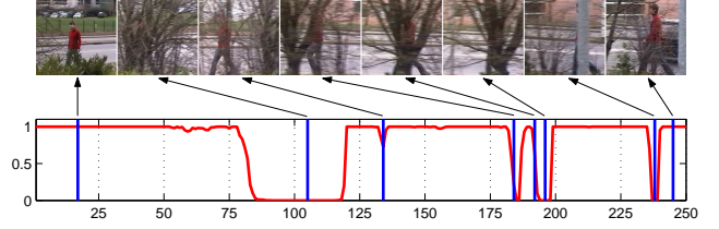
Figure 3. Posterior visibility probability , \xi_{1,t} = p(v_t = 1|y^t) , plotted against time for the example in Fig. 2.
