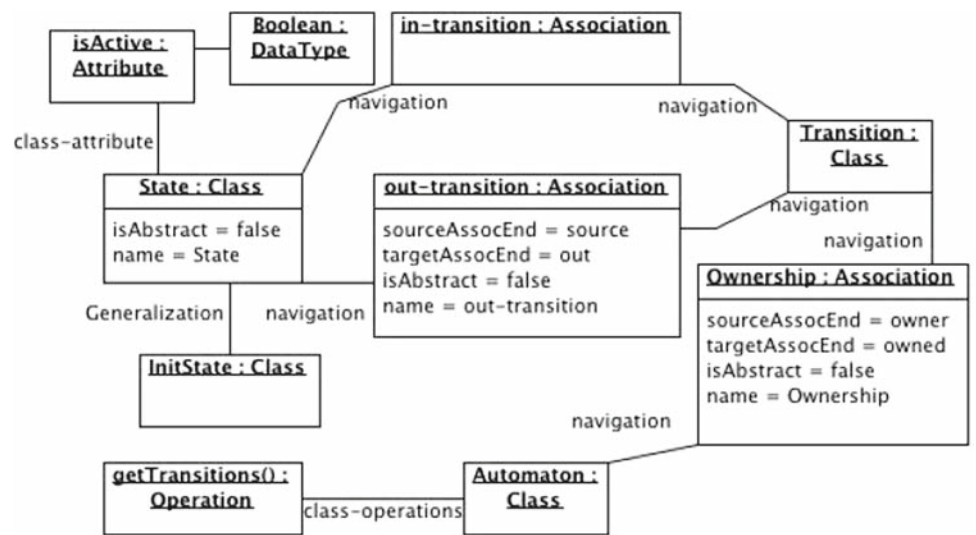
Fig. 3 Model of an automaton as a metamodel instance
