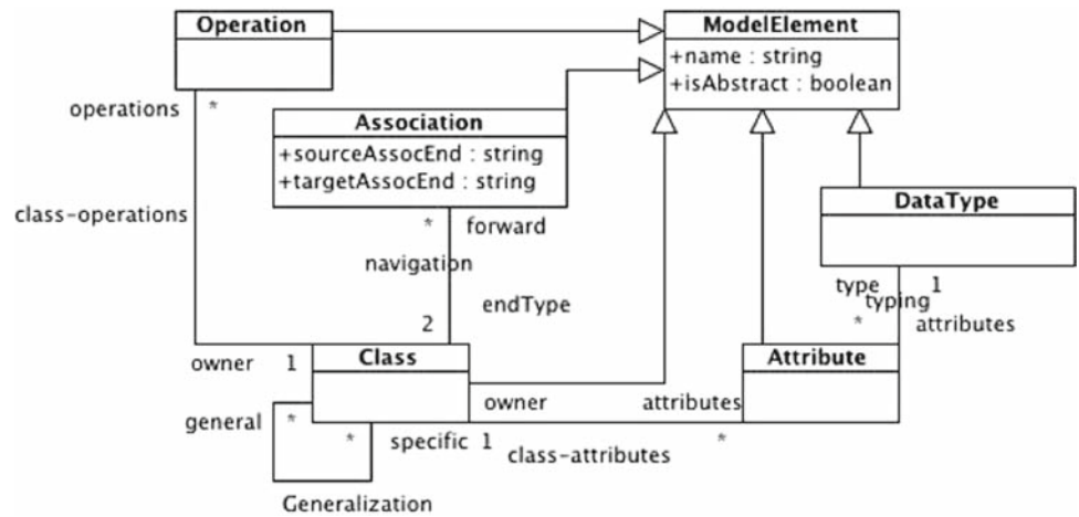
Fig. 1 Basic UML metamodel
