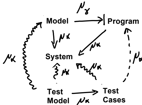
Figure 13: Model-based testing
