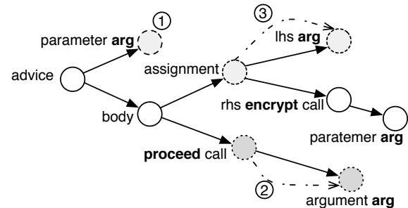
Figure 5. SAST of Encryption aspect, Listing 1, lines 9-12
