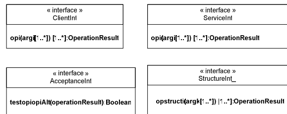
Figure 3 : Recovery Block Aspect Interfaces Class Diagram
