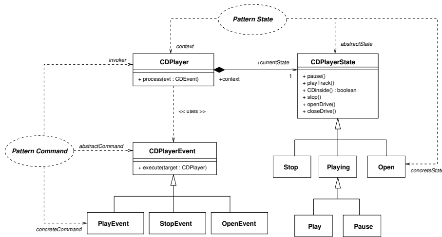
Figure 7: Implementing CD player using states and events reification
