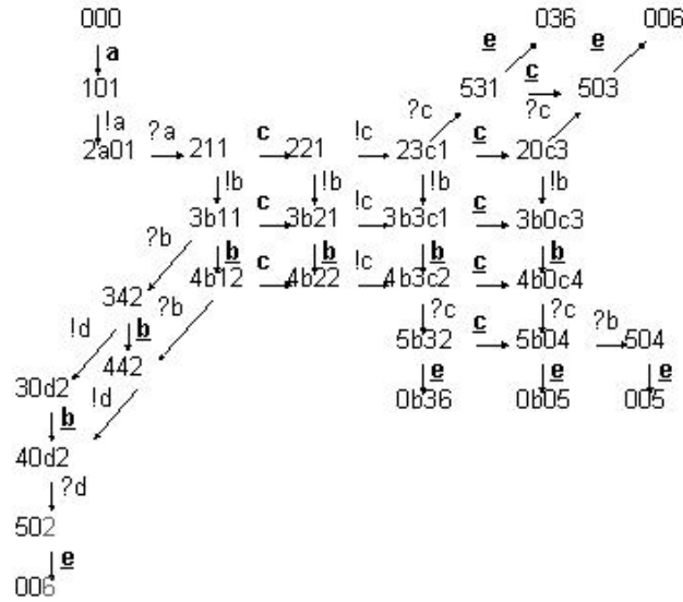
Fig. 6. The state graph of the example
