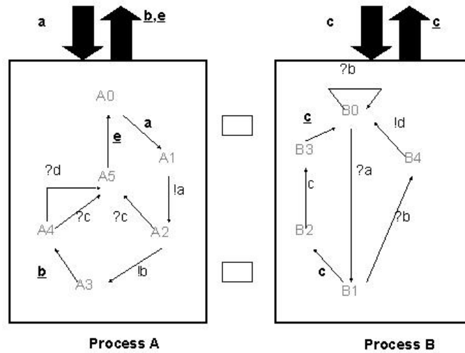
Fig. 1. A small example of connection-disconnection protocol.
