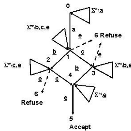
Fig. 5. The “collision” test purpose in TGV
