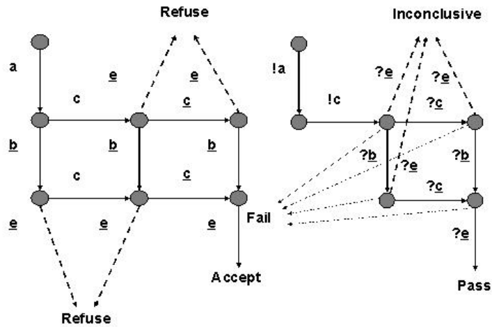
Fig. 7. The abstract state graph (on the left) and the resulting controllable test graph (on the right)
