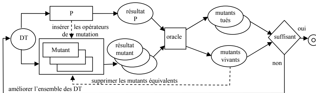
Figure 6 - processus de mutation
