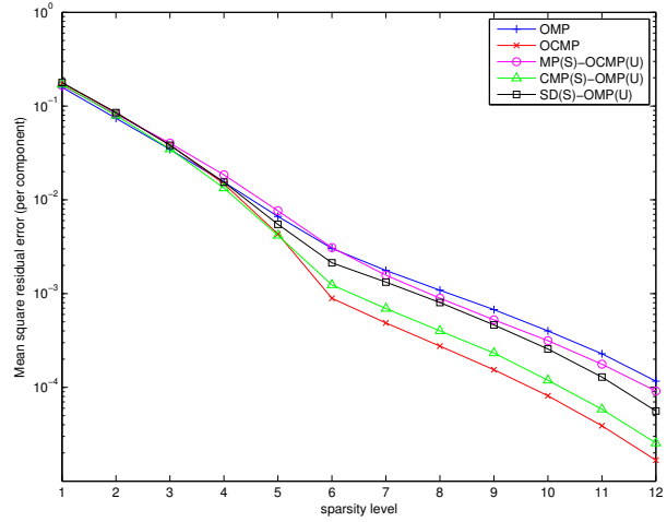
Figure 2: Residual error versus sparsity level. Number of generating atoms is 6. The residual error is computed taking average over 10000 examples. SD(S)-OMP(U) is the pseudo-inverse based sensing dictionary approach.
