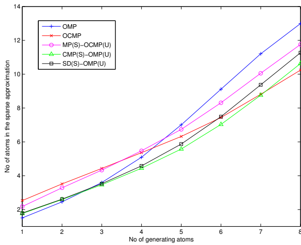
Figure 3: Sparsity of different algorithms with noisy observations. Additive noise is Gaussian with mean 0 and standard deviation 0.001. Residual error bound per component is 0.001. The number of atoms in the approximation is the average over 10000 examples. SD(S)-OMP(U) is the pseudo-inverse based sensing dictionary approach.
