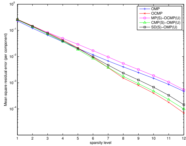
Figure 4: Residual error versus sparsity level with noisy observations. Additive noise is Gaussian with mean 0 and standard deviation 0.001. Number of generating atoms is 6. The residual error is computed taking average over 10000 examples. SD(S)-OMP(U) is the pseudo-inverse based sensing dictionary approach.
