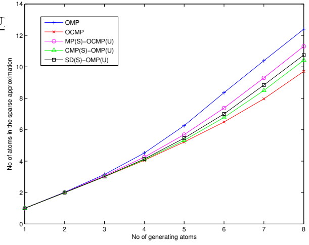
Figure 1: Sparsity of different algorithms. Residual error bound per component is 0.001. The number of atoms in the approximation is the average over 10000 examples. SD(S)-OMP(U) is the pseudo-inverse based sensing dictionary approach.
