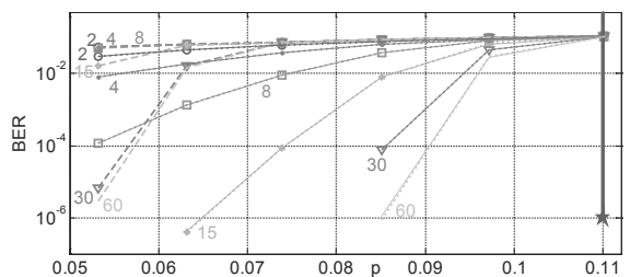
Fig. 3. Comparison of the BER of X for different iterations of the EM.
