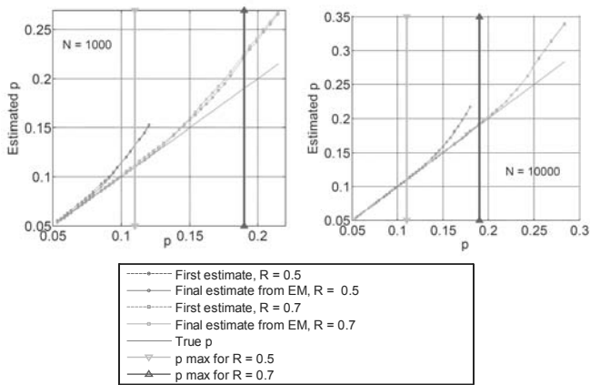
Fig. 1. Means of the estimated \hat{p} in function of N and R .
