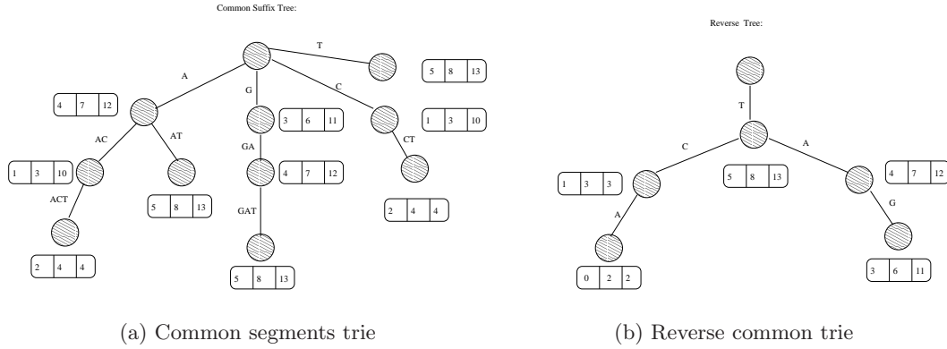
Fig. 3. The common segments trie and the reverse common trie of the example for variable gaps for sequences: S_1 = ACTGAT , S_2 = GTACTTGAT and S_3 = CCACTAGTCACGAT .
