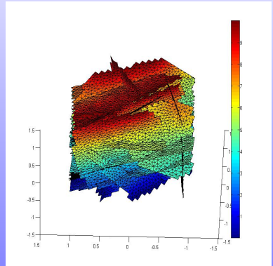
Initial geometry and computed mean pressure
