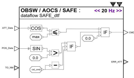
(b) OBSW : On-Board Software model
