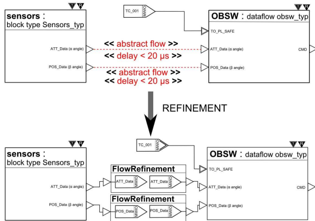
Figure 9: Flow refinement.
