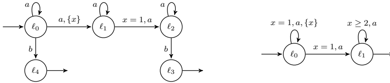
Fig. 10 Examples of determinizable TA not treatable by [BBBB09].
