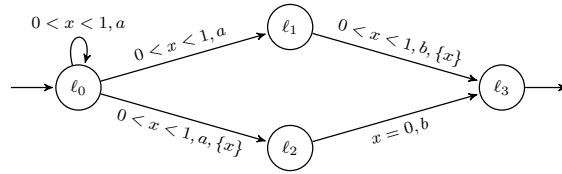
Fig. 1 A timed automaton \mathcal{A} .
