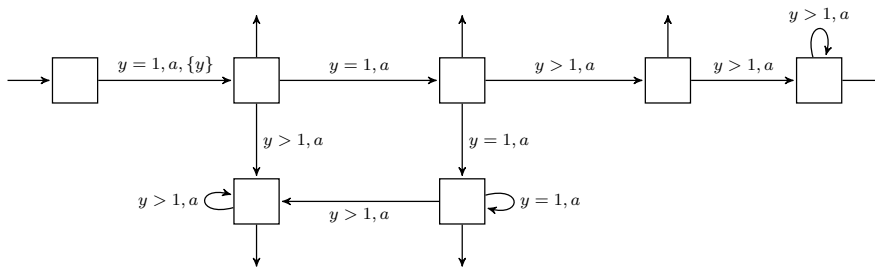
Fig. 11 A deterministic equivalent of the TA of Figure 10, right.
