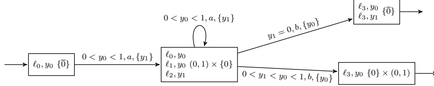
Fig. 12 The result of procedure [BBBB09] on our running example.
