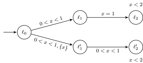
Fig. 15 A timed automaton with invariants.
