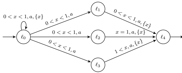
Fig. 7 A determinizable TA for which there is no winning strategy for Determinizator.
