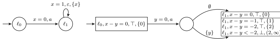
Fig. 13 A timed automaton with \varepsilon -transitions and the resulting \varepsilon -closure.
