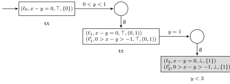
Fig. 16 Excerpt of the game with resources (1, 3) for the TA from Figure 15.
