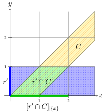
Fig. 4 Construction of the induced guard.
