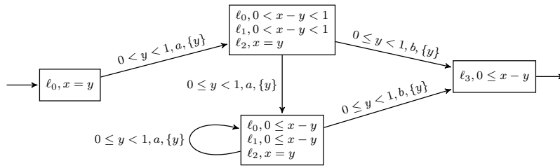
Fig. 9 The result of algorithm [KT09] on the running example.
