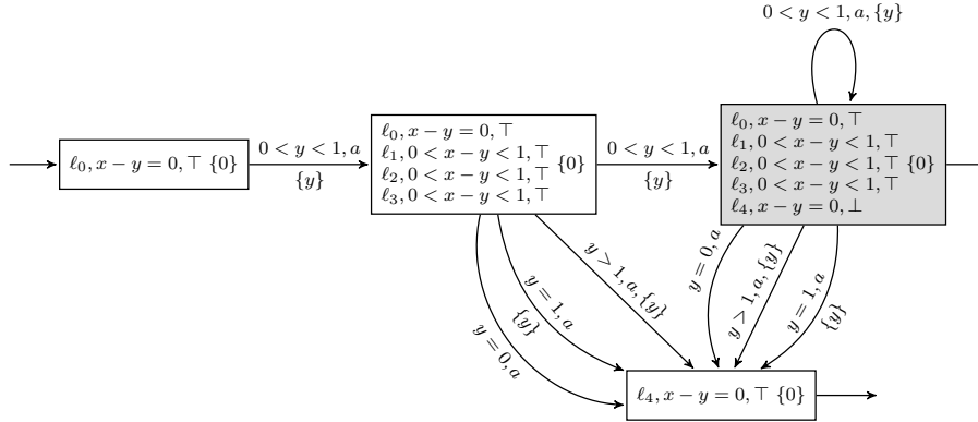
Fig. 8 A deterministic equivalent to the TA in Figure 7 obtained with a losing strategy.
