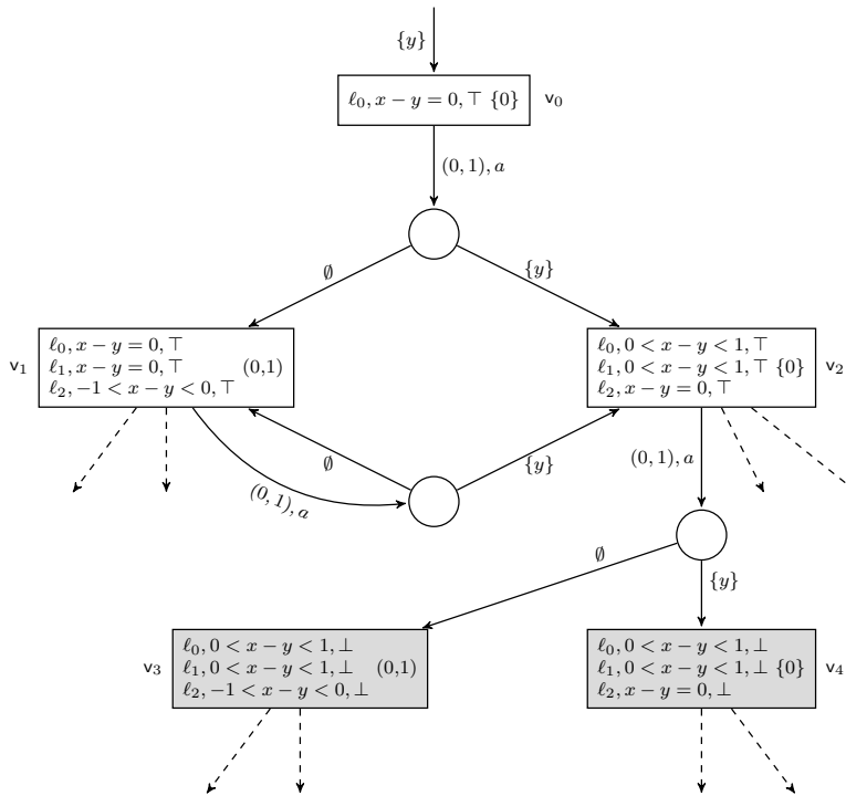
Fig. 3 Excerpt the game \mathcal{G}_{\mathcal{A},(1,1)} .
