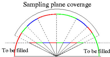
Figure 6: The hemisphere sampling is replaced by rasterizing the scene geometry on a sampling plane. Since this plane does not cover the whole hemisphere, we use a border compensation method to account for the missing directions. Border pixels are extended to avoid zero lighting coming from grazing angles, yielding more plausible results.
