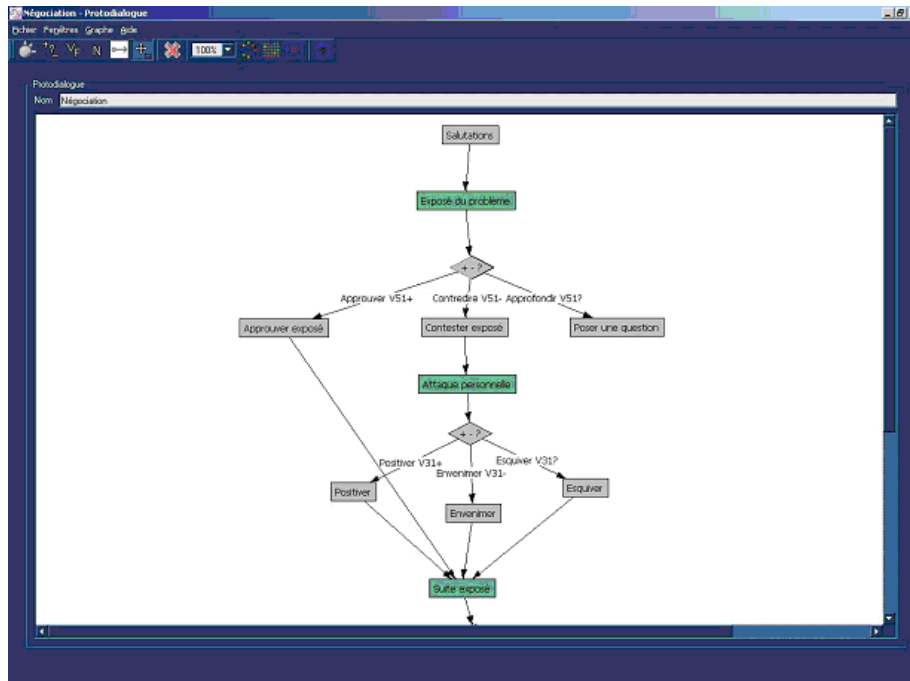
Fig. 5. The Protodialog Edition Window.
