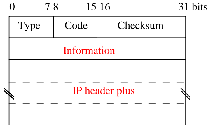
ICMP destination unreachable message
