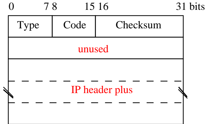
ICMP time exceeded message
