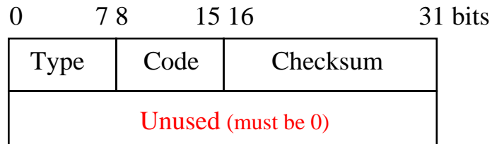
ICMP router solicitation message
