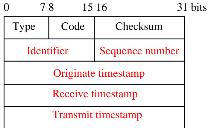
ICMP timestamp message
