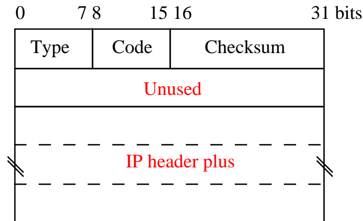
ICMP source quench message
