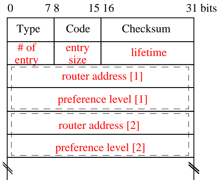
ICMP router advertisement message
