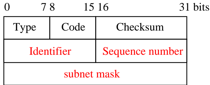
ICMP subnet mask request/reply message
