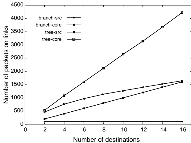
Fig. 22. Control packets overhead in HBH compared to SEM.
