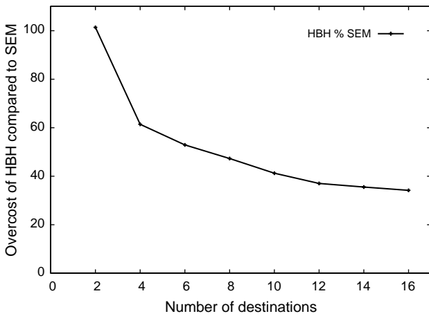
Fig. 21. HBH overhead compared SEM in term of average number of routing states for a channel.
