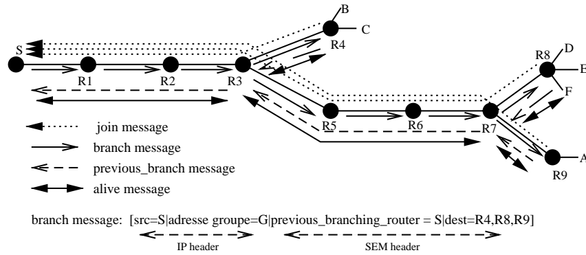
Fig. 5. SEM tree construction.
