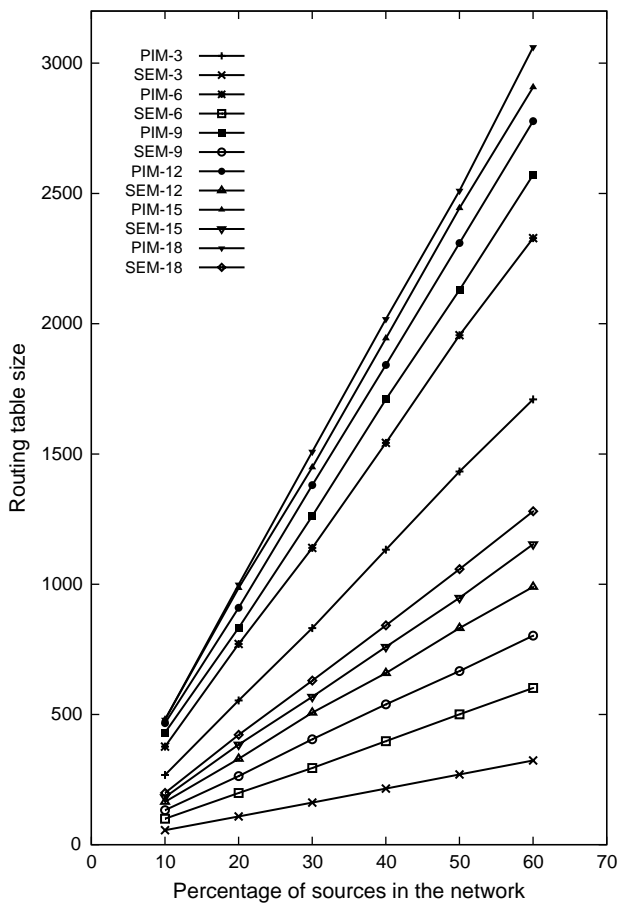
Fig. 18. Global routing tables size per group number in the network—sparse mode and pure random algorithm.
