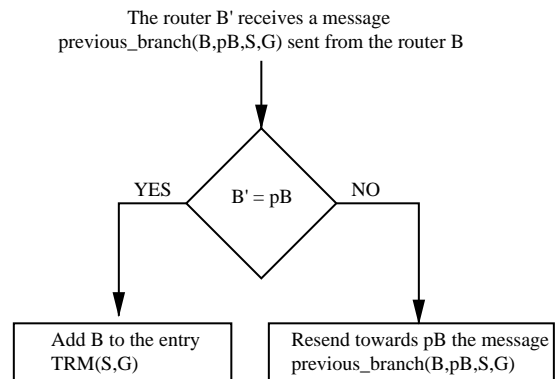
Fig. 4. previous_branch message processing in a SEM router.
