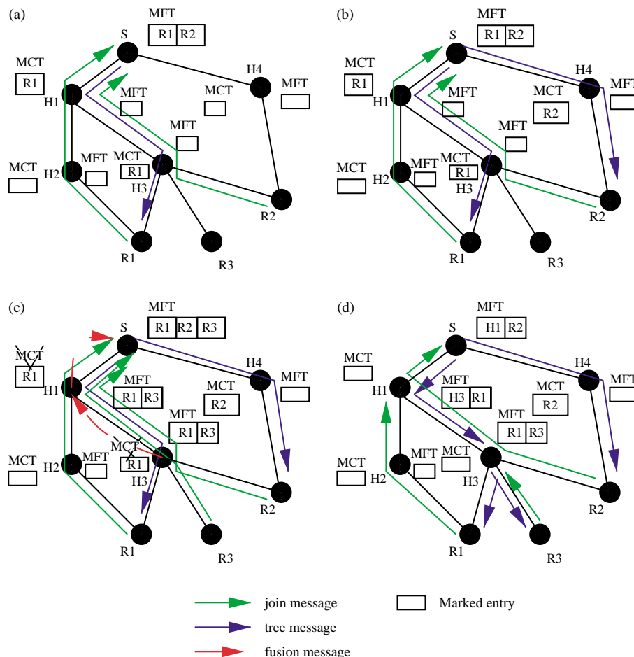
Fig. 10. HBH tree management mechanism.
