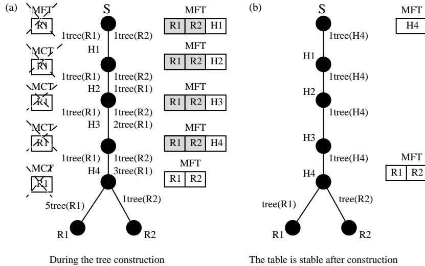
Fig. 16. The tree message in unicast mode.
