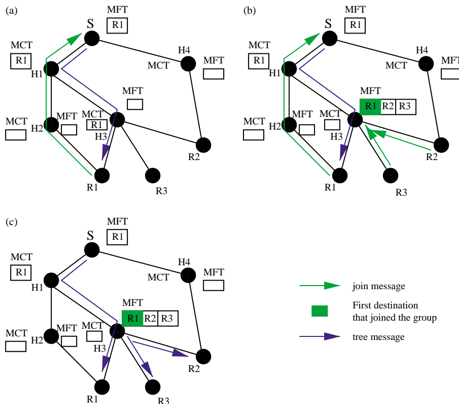
Fig. 8. REUNITE tree management mechanism.
