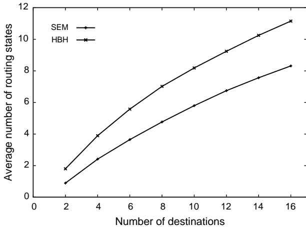
Fig. 20. The average number of routing states for SEM and HBH.
