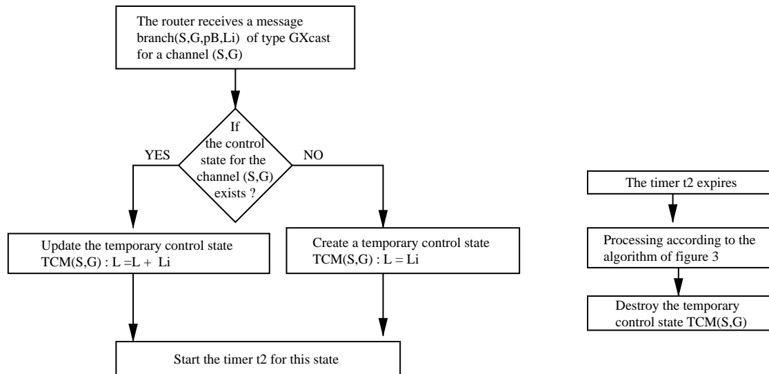
Fig. 12. The processing of a branch message of type GXcast in a SEM router.
