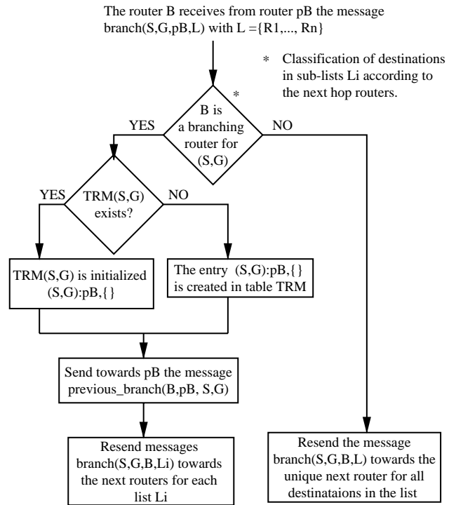
Fig. 3. branch message processing in a SEM router.
