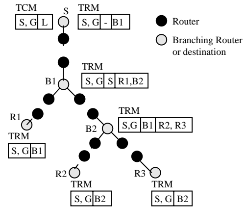
Fig. 1. Multicast routing tables (TRM).
