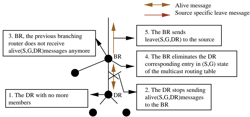
Fig. 6. The case when DR does not have members anymore.
