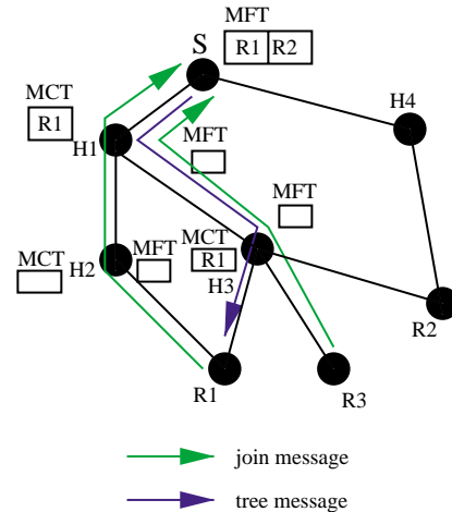
Fig. 15. The tree message in recursive unicast mode.
