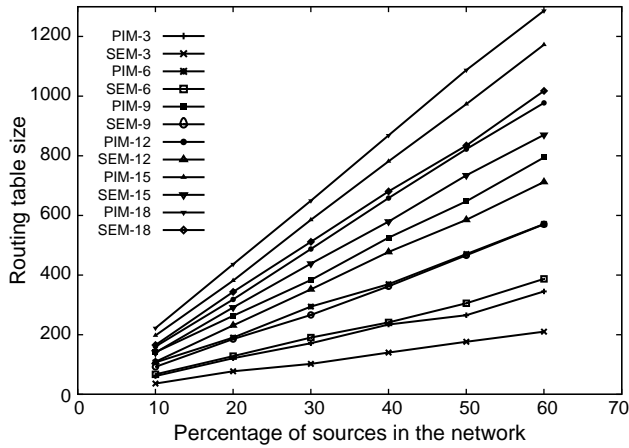
Fig. 17. Global routing tables size per group number in the network—dense mode and Waxman algorithm.
