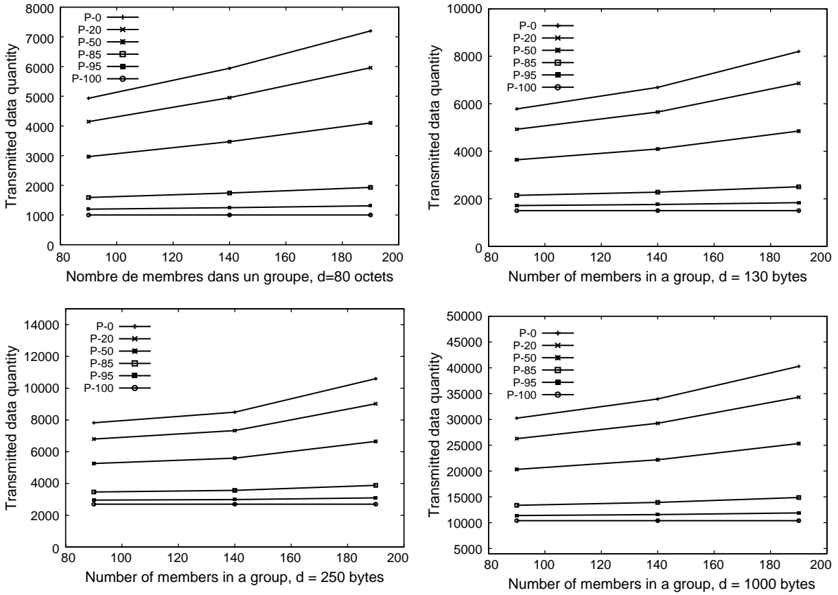
Fig. 23. The transmitted volume in the core network with protocols GXcast and SEM.
