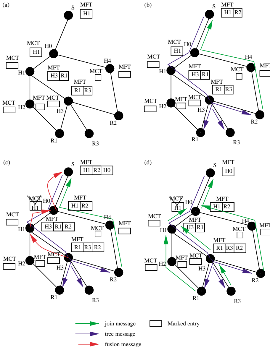
Fig. 14. Comparison of tree states reduction between SEM and HBH.
