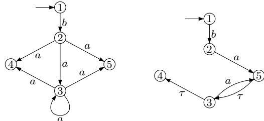
Fig. 5. Process \mathcal{S} and process \mathcal{T}_{\leq}(\mathcal{S})
