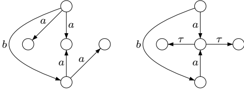
Fig. 3. Generation of nondeterminism in \tau .
