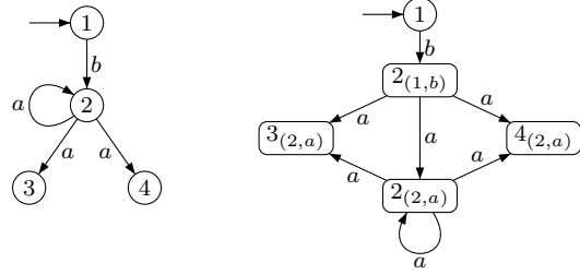
Fig. 4. Process \mathcal{S} and process T_{ip}(\mathcal{S})
