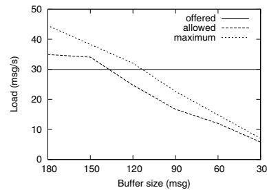
Figure 6. Ideal and adaptive rates.
