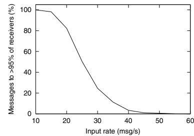
Figure 2. Reliability degradation.
