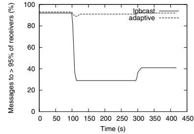
(b) Atomicity.
