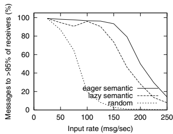
Figure 2. Atomicity of non-obsolete messages.
