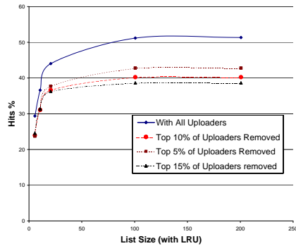
Figure 3: Impact of the removal of u\% of the most generous uploaders
