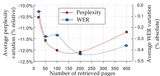
Fig. 2. Influence of the number of pages on perplexity and WER.
