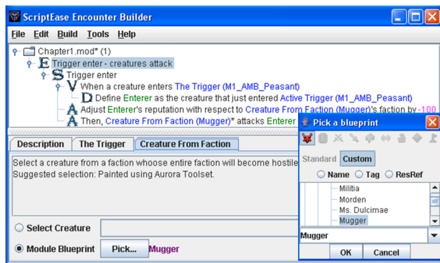
Figure 3. A simple instance of the Trigger enter – creatures attack encounter pattern.
