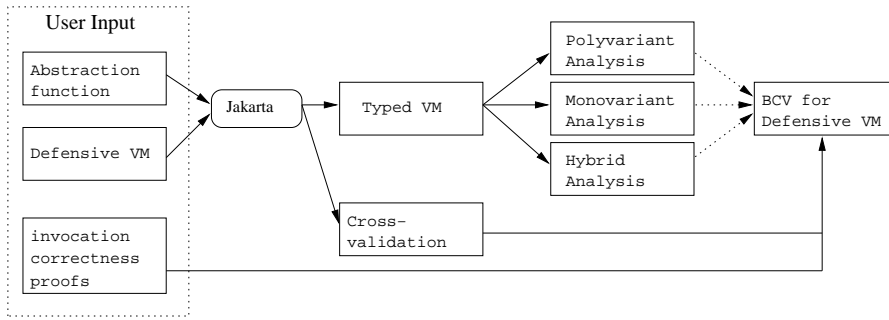
Figure 4. ARCHITECTURE OF THE FW PHASE
