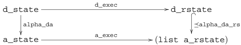
Figure 11. COMMUTATIVE DIAGRAM OF DEFENSIVE AND TYPED EXECUTION
