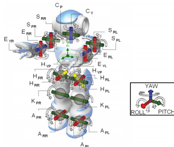
Fig. 1. The Aldebaran NAO robot with its 21 degrees of freedom, and reference frame \mathcal{F}_R ( X , Y , Z ) with origin in the robot center of mass.
