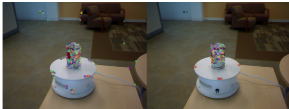
Figure 6: Non-planar object keypoint matching using ORB finds 0 matches.
