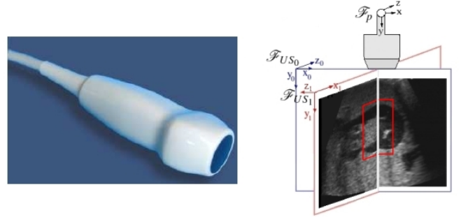
Fig. 4. The XYPA2.5 bi-plane device ( Vernon ) (left) provides two orthogonal US images. The probe frame \mathcal{F}_p is aligned with the frame of the image plane US_0 and the plane US_1 corresponds to a rotation of 90^\circ around the y -axis (right).
