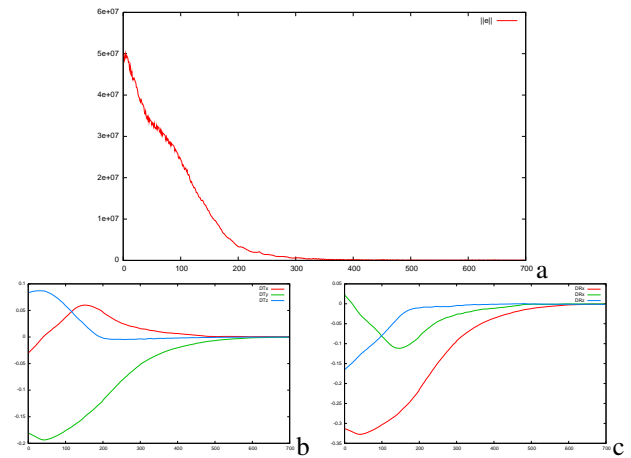
Fig. 7. Stacking luminance and norm of the gradient \mathbf{s} = (\mathbf{I}(\mathbf{r}), \| \nabla \mathbf{I}(\mathbf{r}) \|^2)^T (a) Cost function, (b) Translational part of \Delta \mathbf{r} (m), (c) Rotational part of \Delta \mathbf{r} (rad.)
