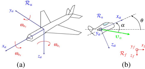
Fig. 1. (a) Aircraft frame and associated rotations, (b) Angles definitions
