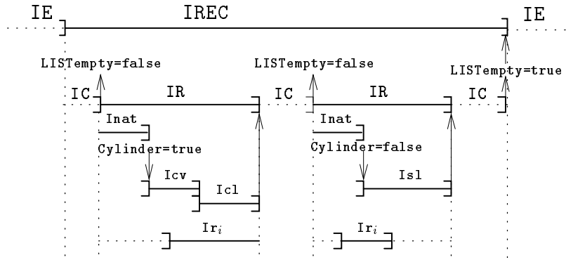
Figure 8: Specification of the sequencing in terms of activity intervals: a possible trace.
