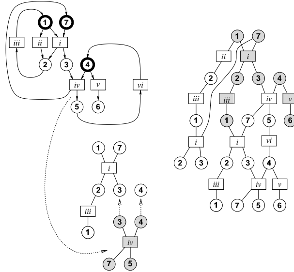
Figure 7: Running example (top left), a configuration (bottom left), and a branching process (right). For this and subsequent examples, we take the following convention for drawing Petri nets and occurrence nets. In Petri nets, the flow relation is depicted using directed arrows . In occurrence nets, since no cycle occurs, the flow relation progresses downwards , and therefore there is no need to figure them via directed arrows, standard solid lines are used instead.
