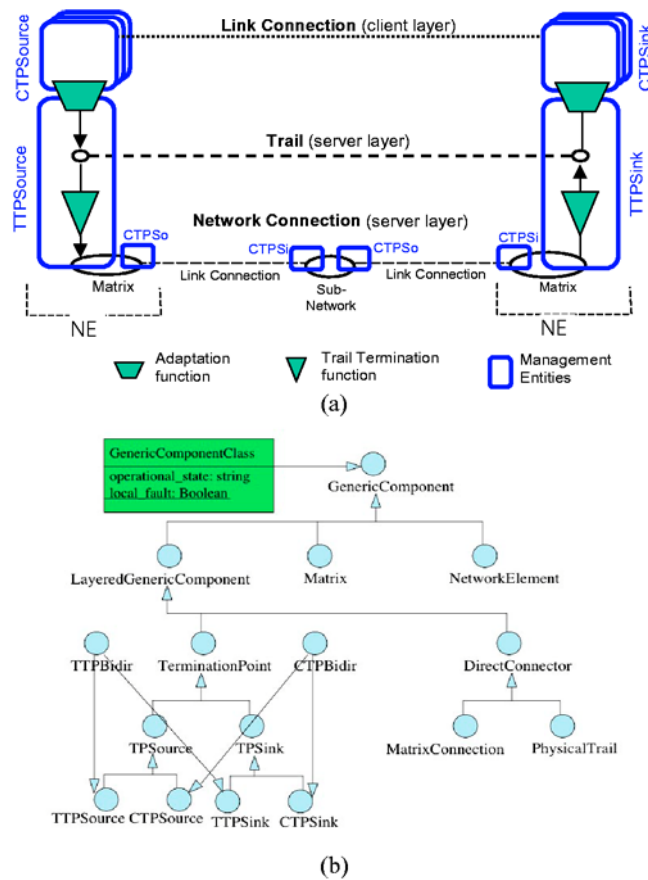
Fig. 1. a. Generic functions and managed entities, b. Generic Components.
