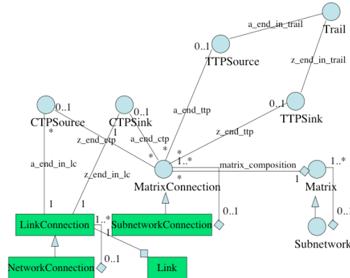
Fig. 2. Peering relations : layer network (horizontal) partitioning.
