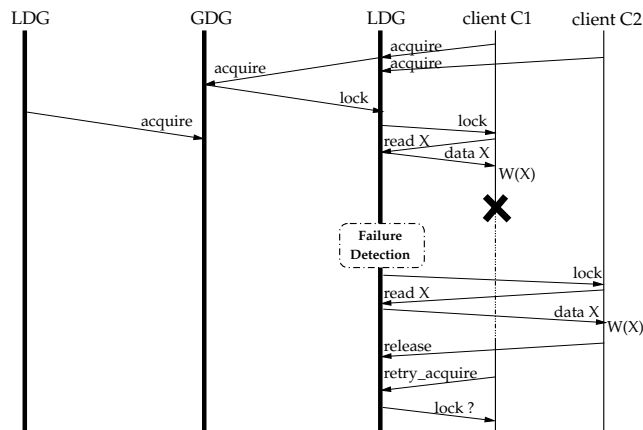
Figure 6. Error of the LDG's failure detector.
