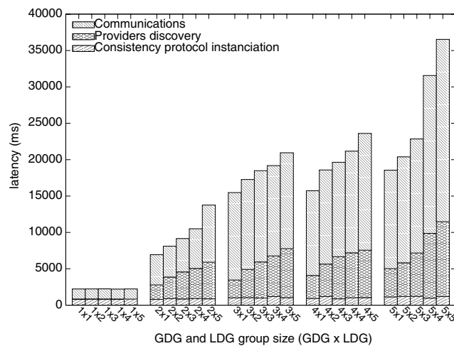
Figure 9. Allocation costs depend on replication degree.
