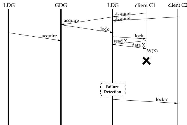
Figure 5. Failure of the exclusive lock owner.
