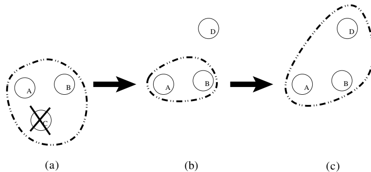
Figure 7. Self-organizing group membership protocols have to replace faulty replicas.
