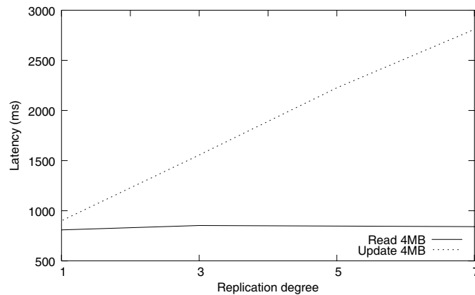
Figure 11. Cost of the basic primitives: 4 MB.
