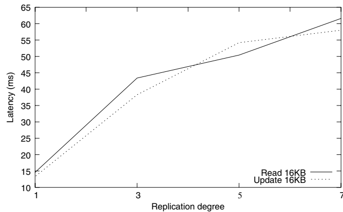
Figure 10. Cost of the basic primitives: 16 KB.
